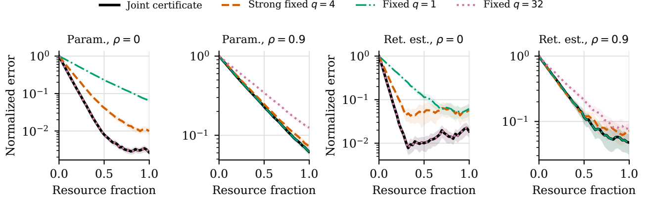
Fig. 4. Held-out resource-indexed convergence in TSP-CURVE-001 for persistence 0.9 and zero delay (64 confirmation seeds; bands are 95 percent confidence intervals). The first two panels show normalized parameter error; the last two show normalized squared error of the fixed-policy discounted-return estimate. The joint Lyapunov certificate changes participation with the dependence regime and improves both learning curves relative to the development-selected strong fixed q = 4 comparator.
