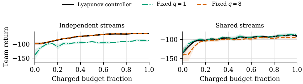
Fig. 5. Preregistered MAPPO team-return learning curves in TSP-MARL-CONF-001 (eight held-out seeds per dependence regime; bands show 95 percent confidence intervals). The fully charged return-free controller commits to fixed q = 8 under independent rollout innovations and fixed q = 1 under shared innovations, tracking the regime-matched fixed action while improving over globally fixed broad participation.
