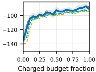
(b) MPE, shared streams
