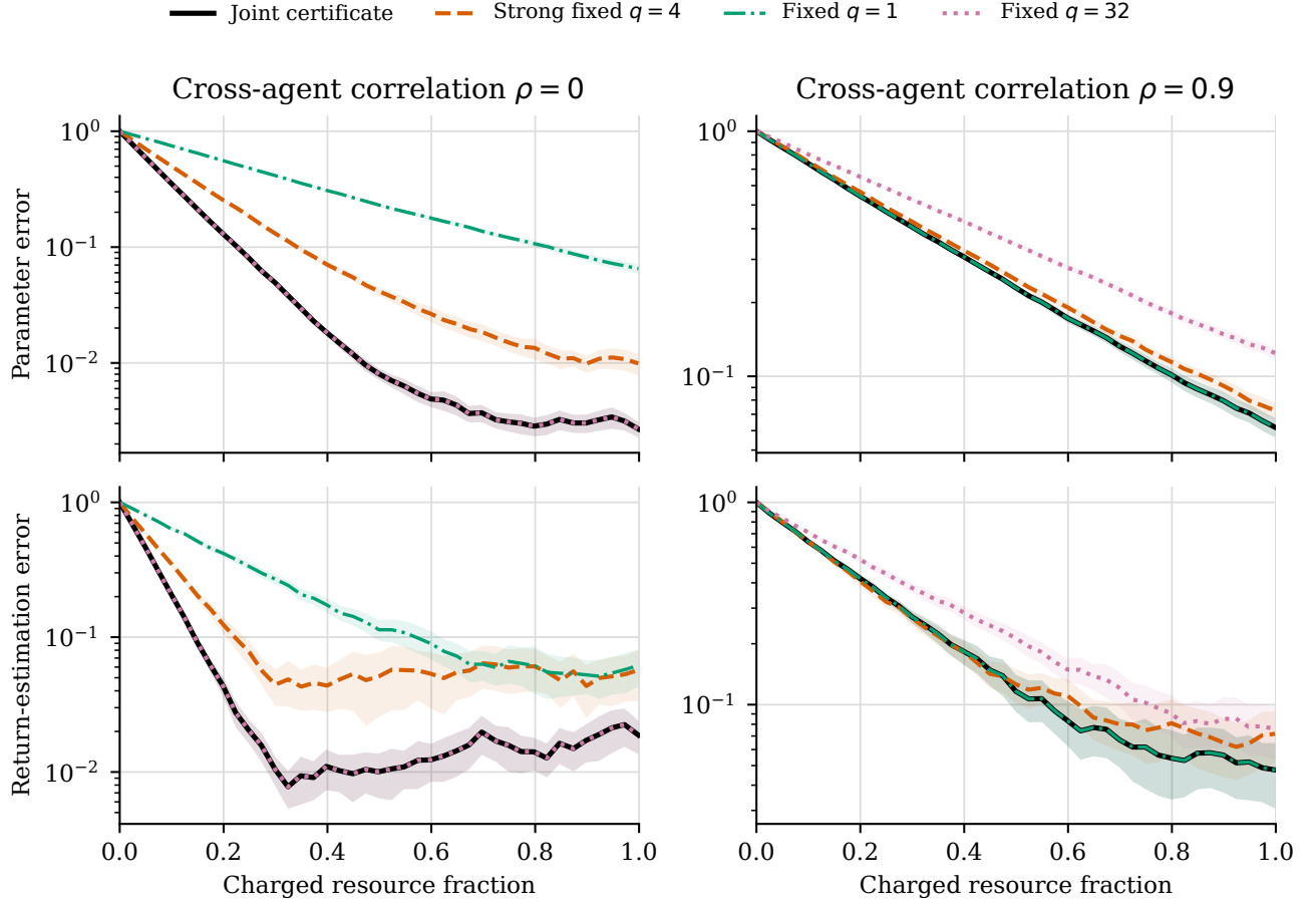
Fig. 4. Held-out resource-indexed convergence in TSP-CURVE-001 for persistence 0.9 and zero delay (64 confirmation seeds; bands are 95 percent confidence intervals). The top row is normalized parameter error and the bottom row is normalized squared error of the fixed-policy discounted-return estimate. The joint Lyapunov certificate changes participation with the dependence regime and improves both learning curves relative to the development-selected strong fixed q = 4 comparator.
