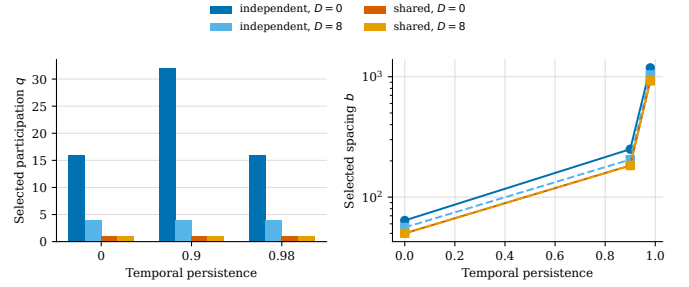
Fig. 2. Joint actions selected by the finite-time Lyapunov certificate in EXP-010B. The left panel reports participation and the right panel reports Markov spacing.
