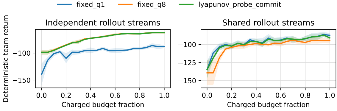
Fig. 5. Preregistered MAPPO team-return learning curves in TSP-MARL-CONF-001 (eight held-out seeds per dependence regime; bands show 95 percent confidence intervals). The fully charged return-free controller commits to fixed q = 8 under independent rollout innovations and fixed q = 1 under shared innovations, tracking the regime-matched fixed action while improving over globally fixed broad participation.
