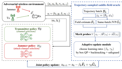
Fig. 3. LCMPL minimax policy-learning framework.
