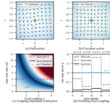
Fig. 1. Why saddle-field step sizes must adapt to local coupling. For the local update \mathbf{z}_+ = \mathbf{z} - \beta \mathbf{F}_\omega(\mathbf{z}) + \gamma \nabla \mathbf{F}_\omega(\mathbf{z}) \mathbf{F}_\omega(\mathbf{z}) , \omega denotes coupling strength, \beta and \gamma are the field and curvature step sizes, and q = \|\mathbf{z}_+\|/\|\mathbf{z}\| is the one-step norm ratio. Panels (a) and (b) show the rotational field action and inward Jacobian–field action. Panel (c) shows that the contraction region q < 1 and its locally minimizing curvature-to-field ratio \gamma/\beta vary with \omega . Panel (d) follows switching coupling: a fixed ratio crosses q = 1 , whereas the local ratio remains contractive.
