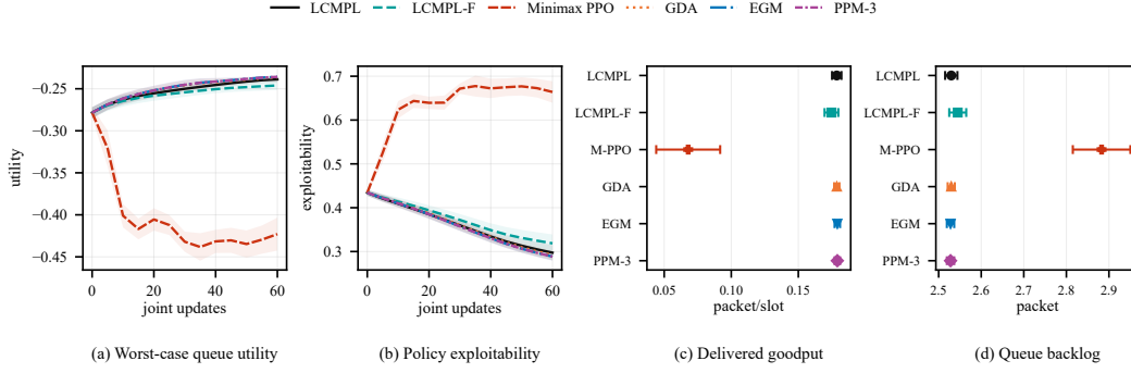
Fig. 4. Queue-aware nominal benchmark at moderate load over 12 seeds. Curves show means with one standard error; points show final means with 95% confidence intervals.
