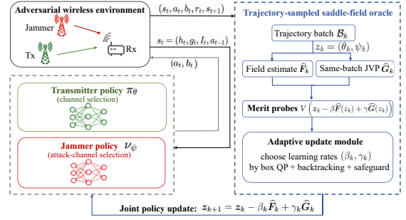
Fig. 3. LCMPL minimax policy-learning framework.
