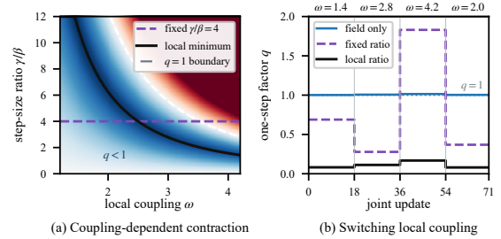
Fig. 1. Why saddle-field step sizes must adapt to local coupling. For a scaled bilinear local model, (a) maps the one-step residual factor q over coupling \omega and the field-to-curvature step-size ratio. The contraction region q < 1 and its locally minimizing ratio vary with coupling. Panel (b) follows a switching coupling sequence; a fixed ratio crosses the q = 1 boundary, whereas the local ratio remains contractive.
