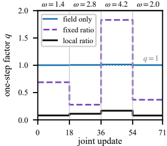
(b) Switching local coupling
