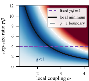
(a) Coupling-dependent contraction
