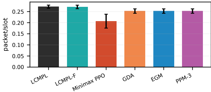
(c) Delivered goodput
