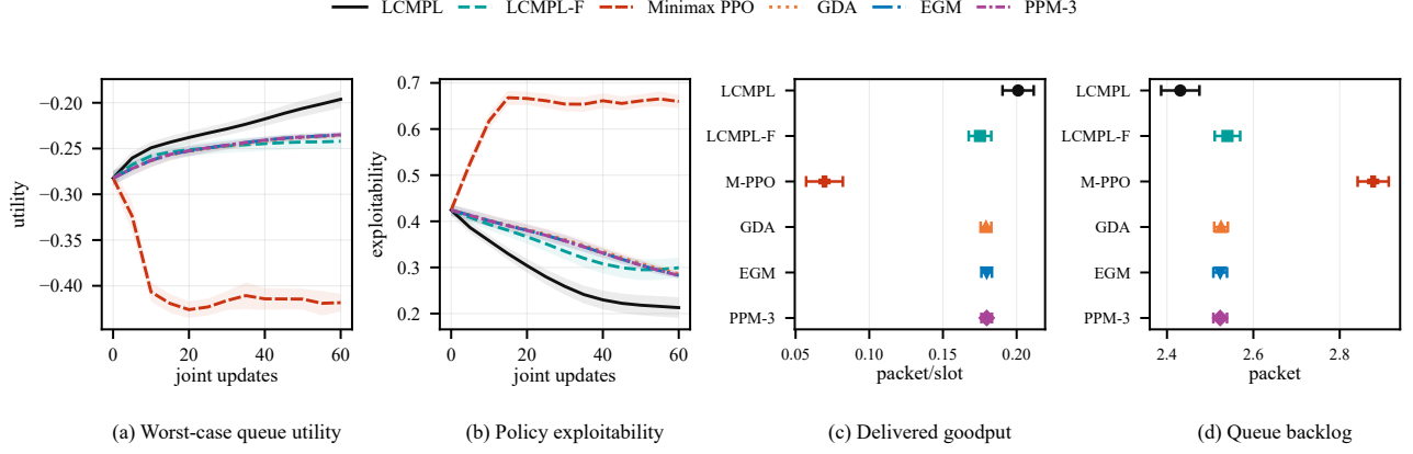
Fig. 4. Queue-aware nominal benchmark at moderate load over 12 seeds. Curves show means with one standard error; points show final means with 95% confidence intervals.
