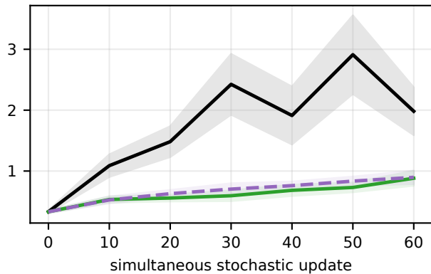
batch 128: population field norm (lower is better)
