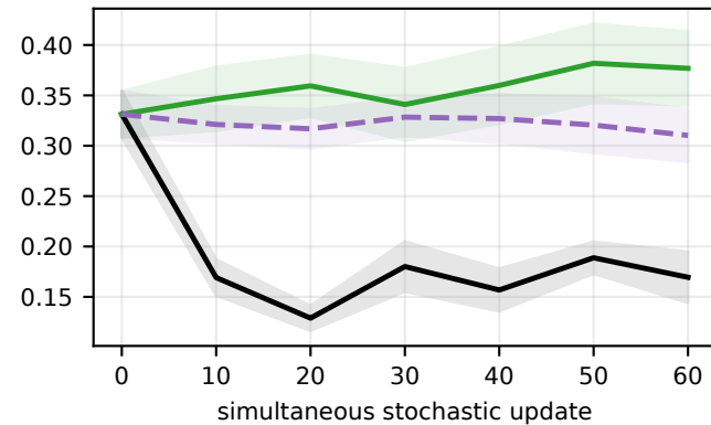
batch 2048: population field norm (lower is better)
