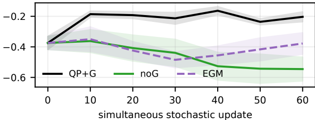
hard-BR return (higher is better)
