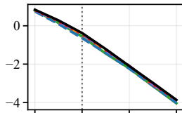
SecurityPatrol
