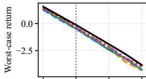
CyclicControl
