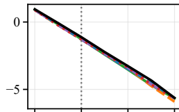
RoutingInterdiction
