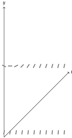
Figure 5: The slopen field for the equation \frac{dy}{dt} = \frac{1}{2} (1 - y) y
