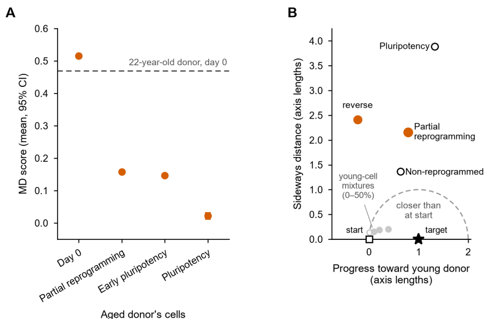
Figure 1. A published aging score falls while the cells move away from young cells. (A) MD score in the aged donor's cells by state, mean and 95% bootstrap interval over cells, with both donors scored against the same control genes. The dashed line is the 22-year-old donor's day-0 fibroblasts: the same score applied to cells that really are young. (B) The same cells in the 205 MD genes, drawn in the plane spanned by the line from the aged donor's day-0 cells (square, at 0) to the young donor's day-0 cells (star, at 1) and the direction perpendicular to it, in units of that line's length. Points inside the dashed circle are closer to the young target than the starting point was. Gray points are young-cell mixtures (0 to 50% young cells; open, 0%); the reverse test is drawn in its own frame with the donors swapped. Donors are never pooled.
