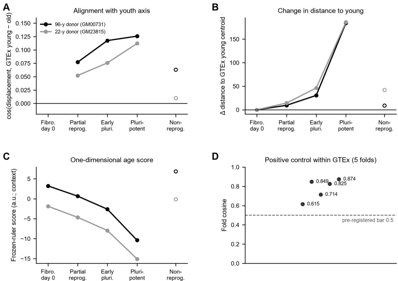
Supplementary Figure S1. Reprogramming states against a GTEx-defined youth axis, all genes. (A) Cosine between each state's displacement from day-0 fibroblasts and the GTEx young-minus-old direction. (B) Change in Euclidean distance to the GTEx young centroid; positive is farther. (C) The frozen ruler score of each state, shown as context. (D) Positive control: the 652 GTEx fibroblast donors were split into five folds; in each fold, held-out old donors were displaced toward that fold's young centroid. Open symbols in A to C are non-reprogrammed cells (OSKM-exposed cells that remained off the reprogramming path), not a second day-0 sample. Donors are never pooled; the 22-year-old donor is a contrast, not a replicate.
