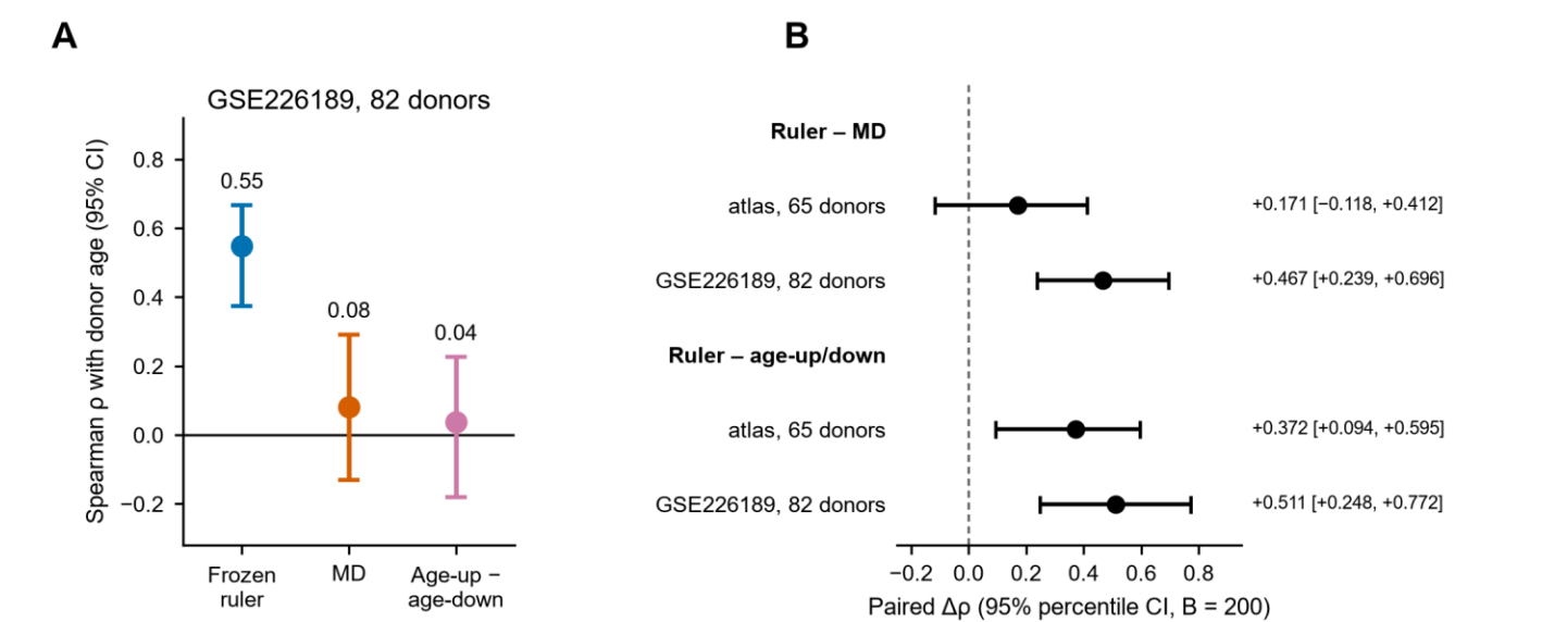
Figure 4. The frozen ruler against two curated instruments. (A) Spearman \rho with donor age for each instrument in GSE226189, with 95% percentile bootstrap intervals. (B) Paired \Delta p (ruler minus the other instrument). Against MD, the atlas interval includes zero.
