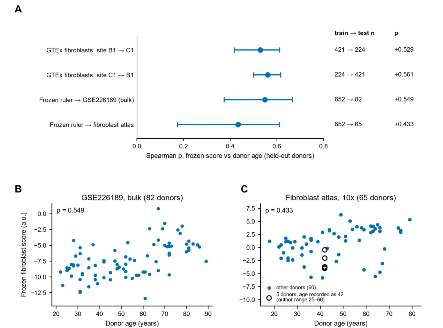
Figure 3. Transfer of the frozen fibroblast ruler. (A) Spearman \rho with donor age for every transfer in Table 1, with 95% percentile bootstrap intervals from 200 resamples of donors. (B) GSE226189 bulk cohort, 82 donors. (C) Dermal fibroblast atlas, 65 donors. Repeated samples from the same person are averaged; the 23 accessions from five donors of one constituent study, whose age is recorded as 42 but reported by the source authors only as 25 to 60 years, are drawn as open circles.
