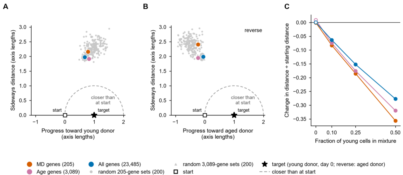
Figure 2. The result does not depend on which genes are read. (A) The test drawn as in Figure 1B for the MD genes (205), the published age-up and age-down genes (3,089) and all genes of the reference panel (23,485), with 200 random gene sets of each of the two smaller sizes matched on expression level and detection. Points inside the dashed circle are closer to the young target than the starting point was. (B) The reverse test, with the donors swapped. (C) Young-cell mixtures in the three gene spaces: change in distance to the young target divided by the starting distance, against the fraction of young cells mixed in; open symbols are the zero-mixture noise floor. No gene set ends inside the circle in A or B, and every gene set registers the mixtures as moving closer in C.
