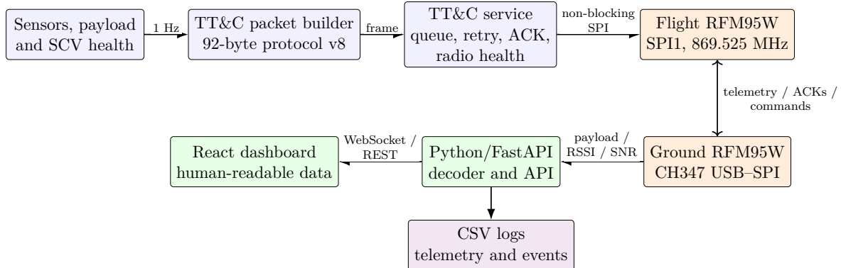
Figure 4.1: End-to-end TT&C architecture and ownership boundaries.
