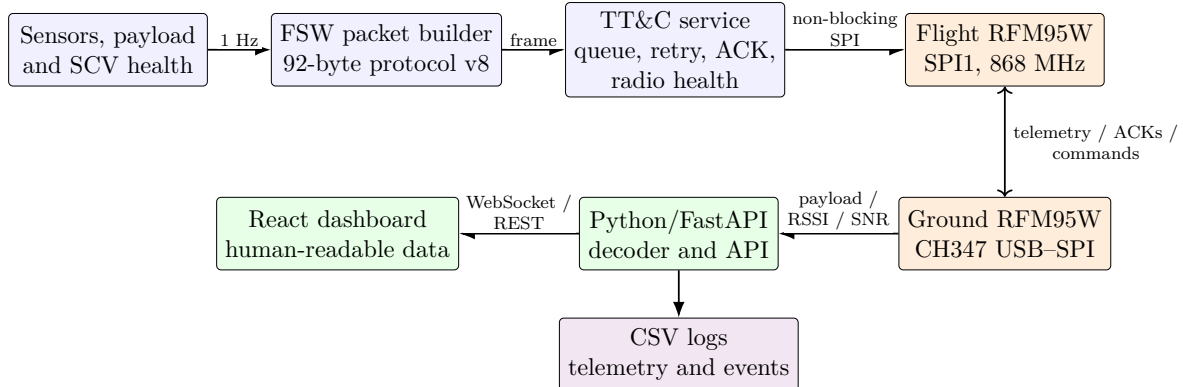
Figure 4.1: End-to-end TT&C architecture and ownership boundaries.
