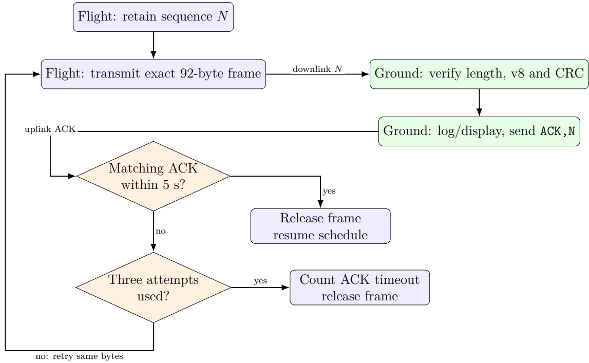
Figure 4.3: Application-level acknowledgement and retry sequence.
