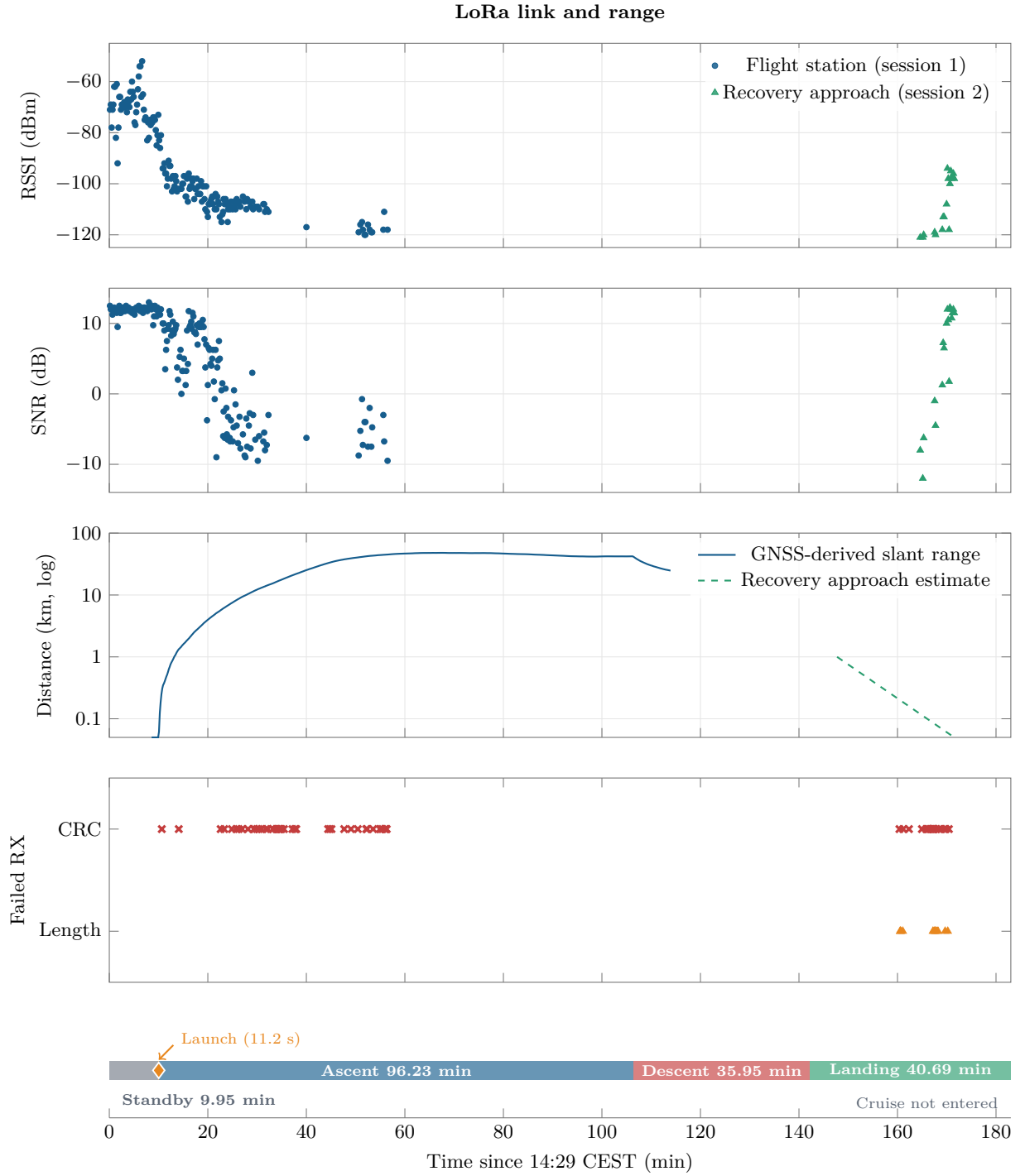
Figure 7: LoRa link and range.
