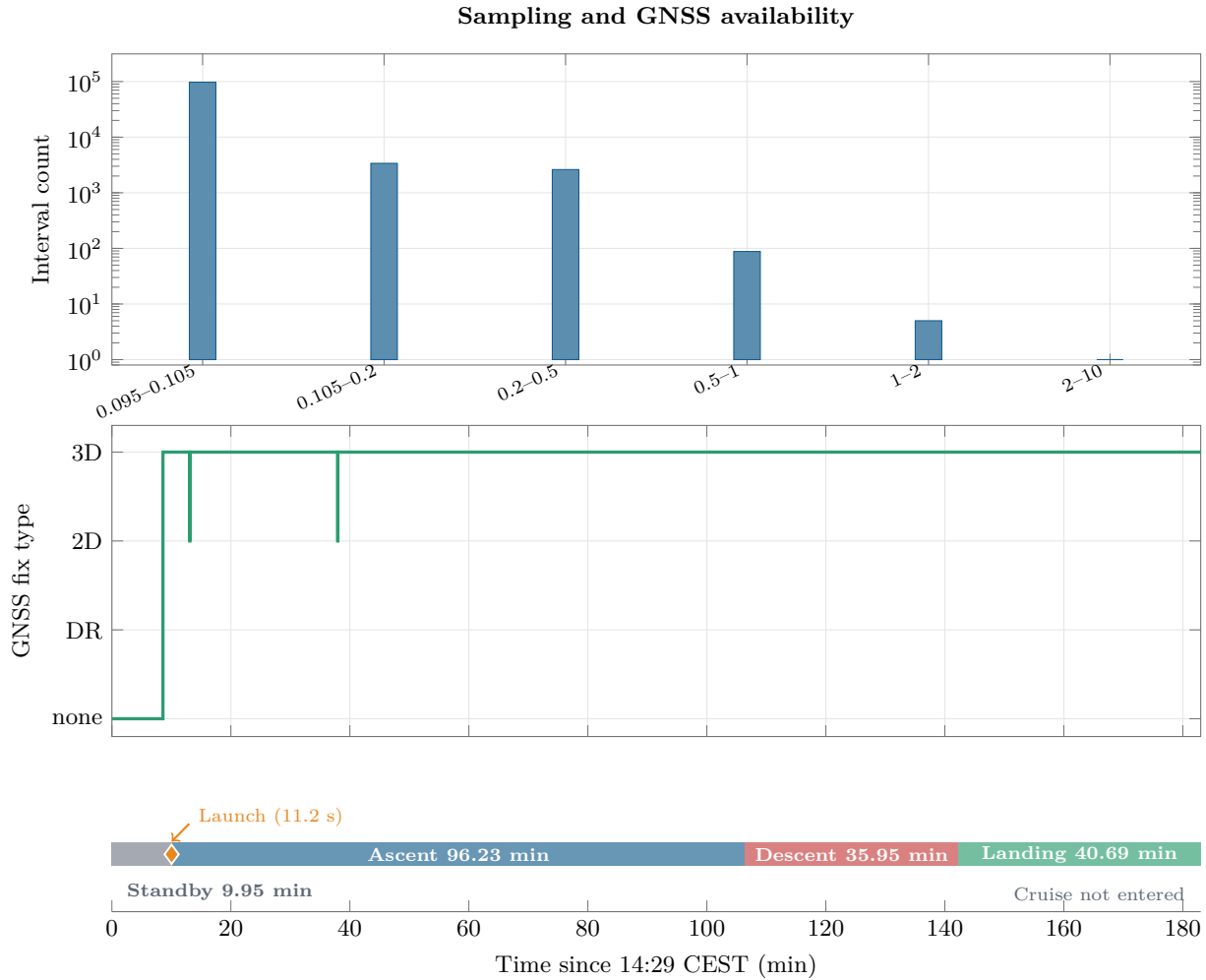
Figure 8: Sampling and GNSS availability.
