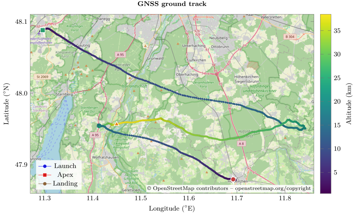
Figure 4: GNSS ground track.
