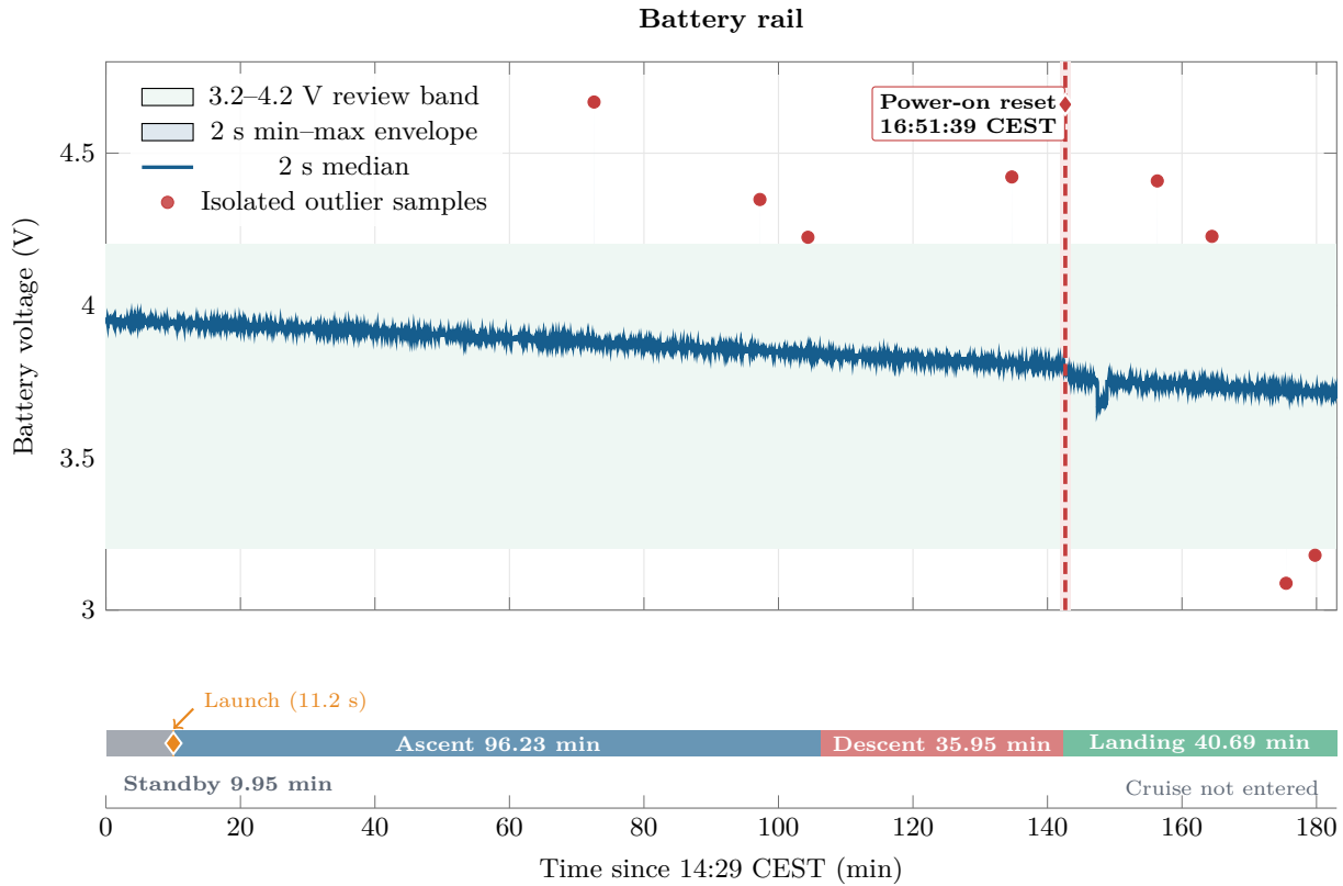
Figure 5: Battery rail.
