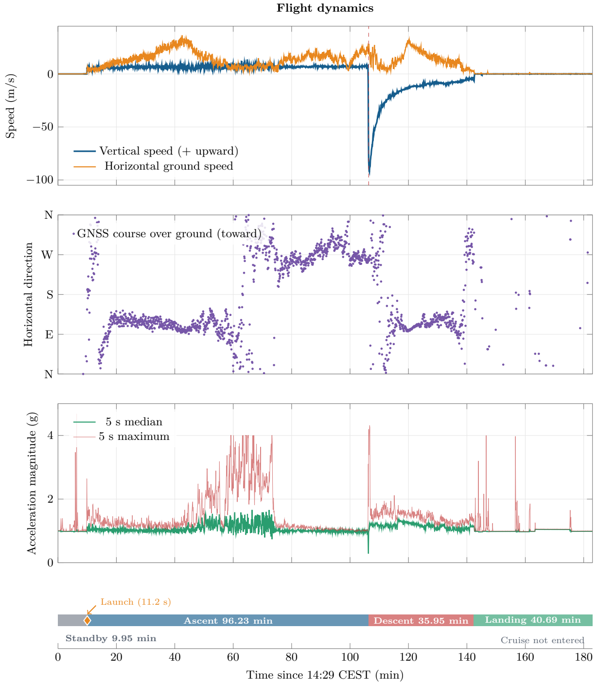
Figure 2: Flight dynamics.
