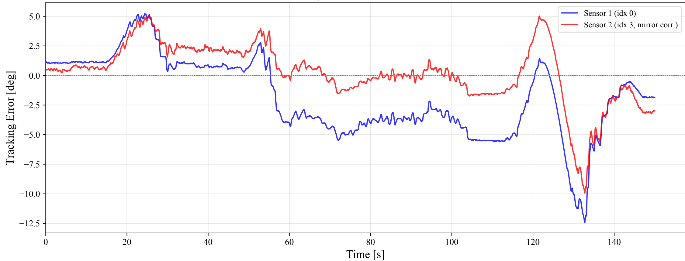
System 1: Tracking Error (RMSE: S1=3.786°, S2=2.515°)
