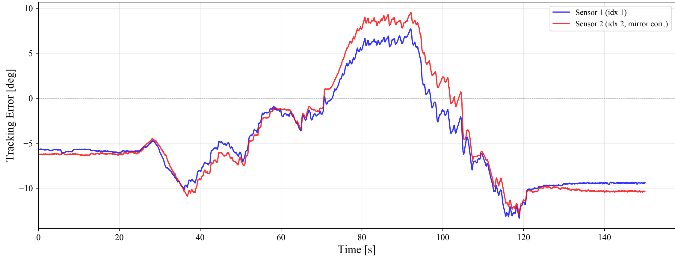
System 2: Tracking Error (RMSE: S1=6.938°, S2=7.448°)
