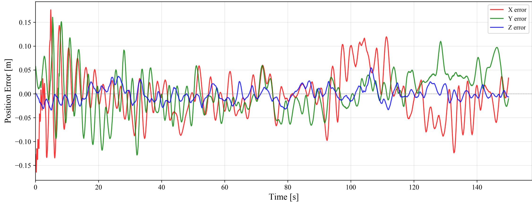
UAV Position Error (RMSE: X=0.0492m, Y=0.0444m, Z=0.0150m)
