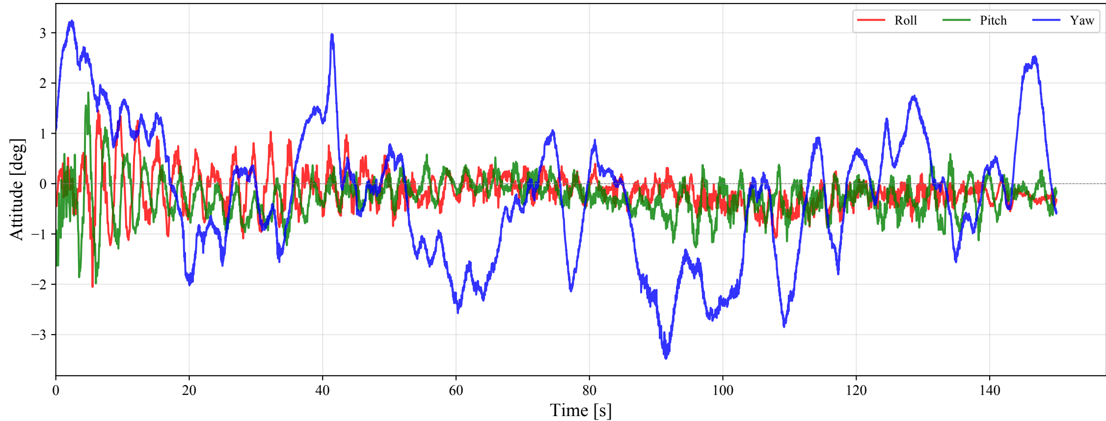
UAV Attitude (Std: Roll=0.360°, Pitch=0.378°, Yaw=1.347°)
