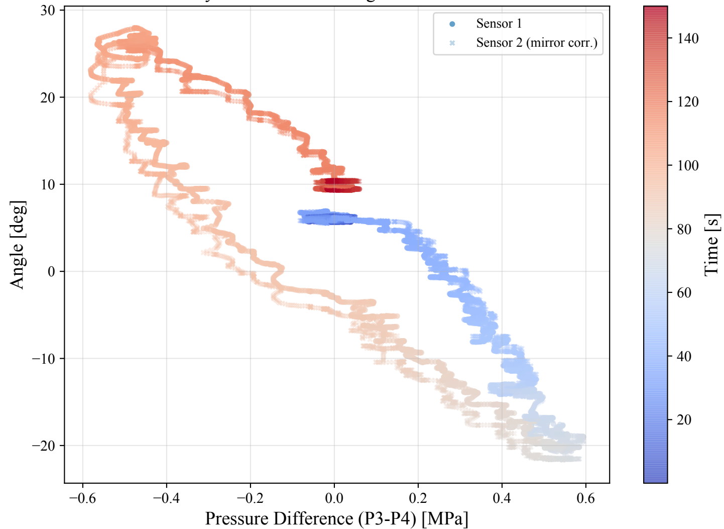
System 2: Pressure-Angle Correlation
