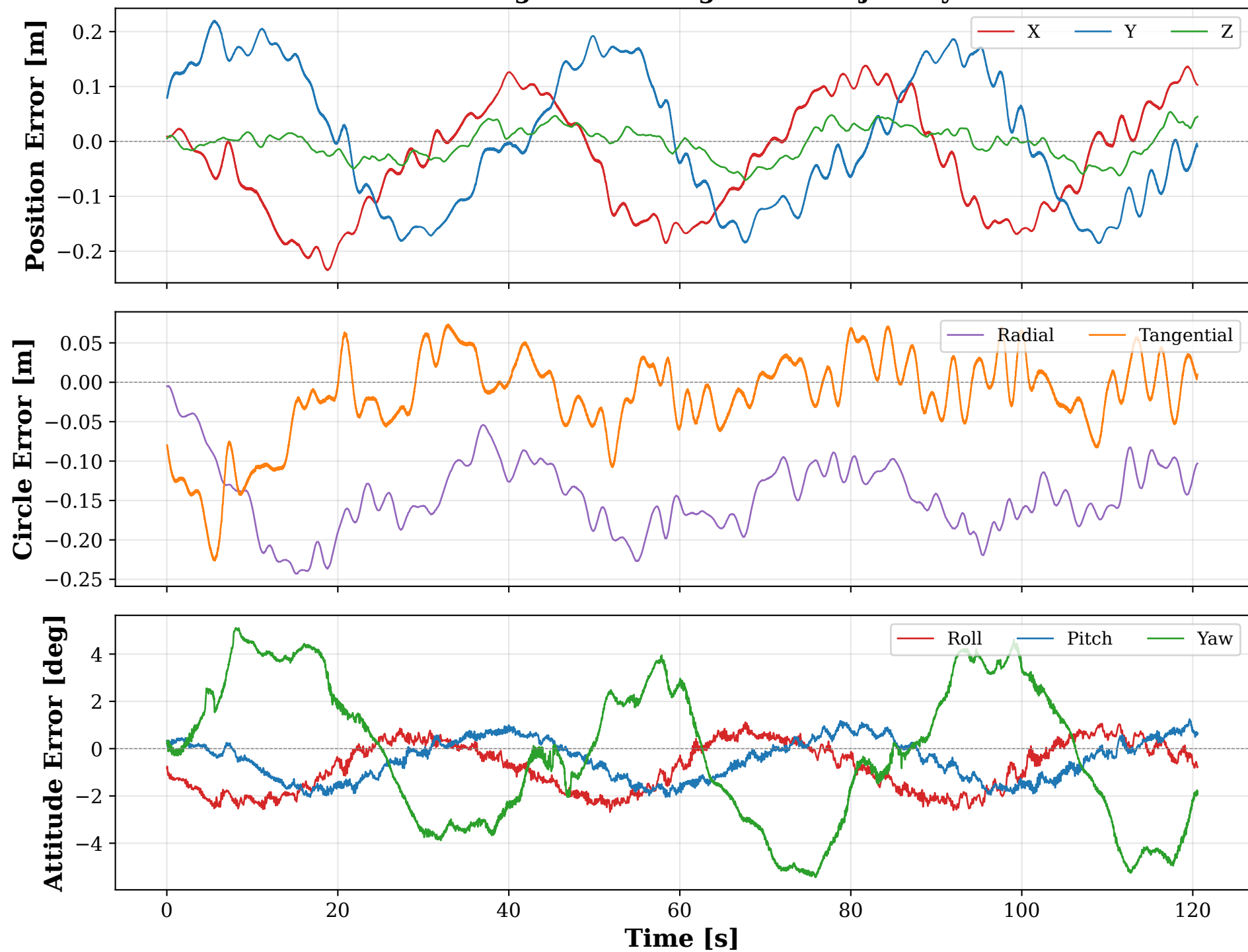
Tracking Error during Circle Trajectory
