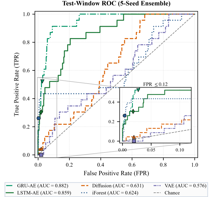
Fig. 2. Test-window receiver operating characteristic (ROC) curves for the 5-seed ensemble models on CAISO data, GRU-AE (downward triangle), LSTM-AE (diamond), Diffusion (upward triangle), iForest (circle), VAE (square), with the inset showing the operational low-false-positive region (false positive rate \text{FPR} \leq 0.12 ).
