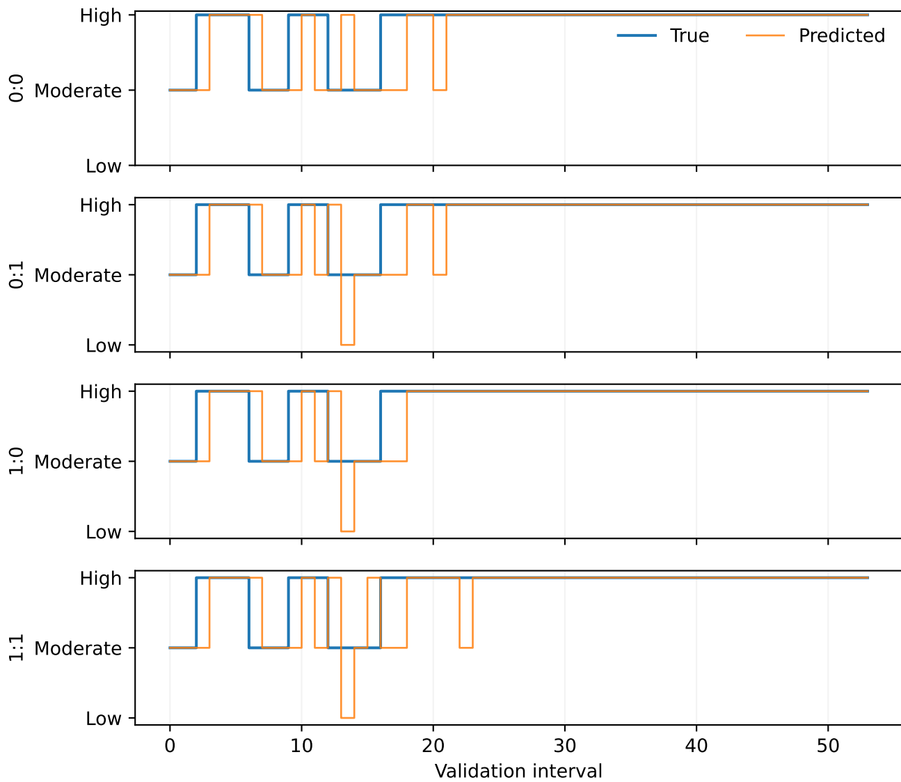
Set 3 memory/off-core per-core timelines
