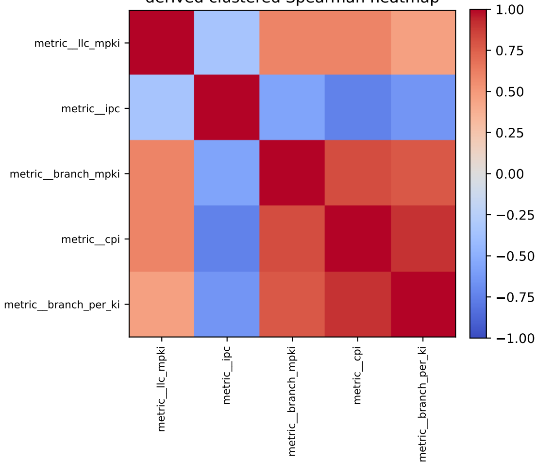
derived clustered Spearman heatmap
