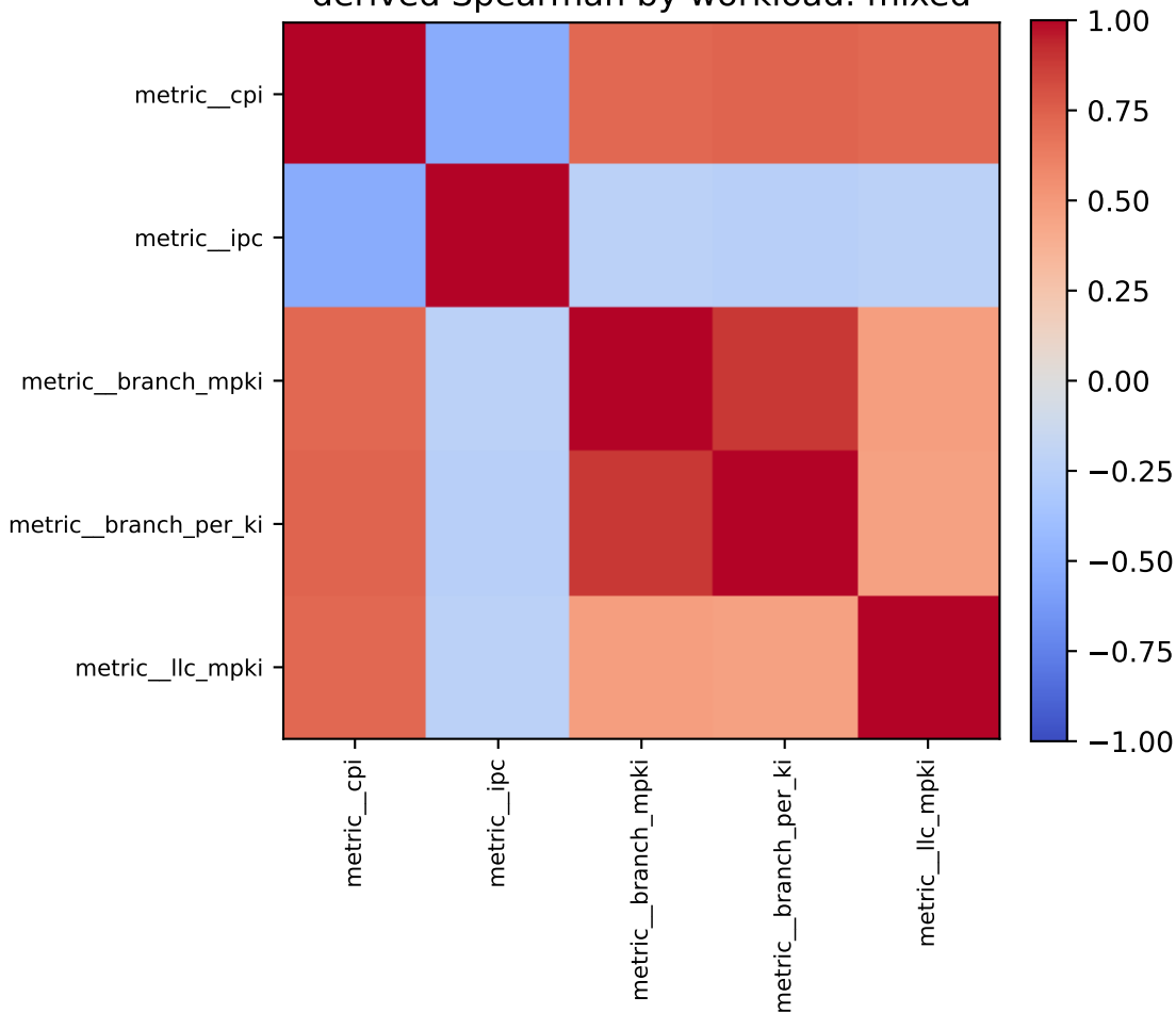
derived Spearman by workload: mixed
