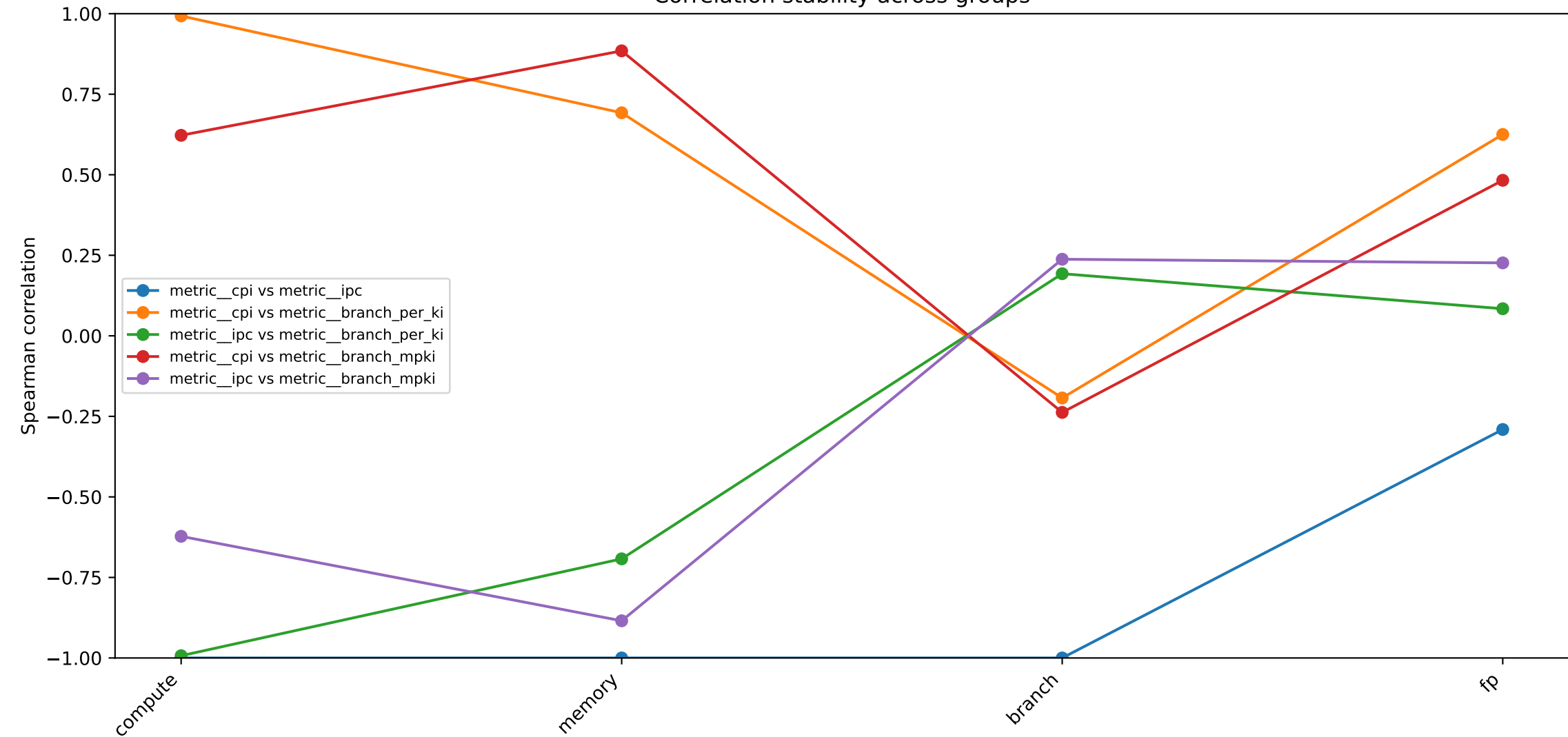
Correlation stability across groups
