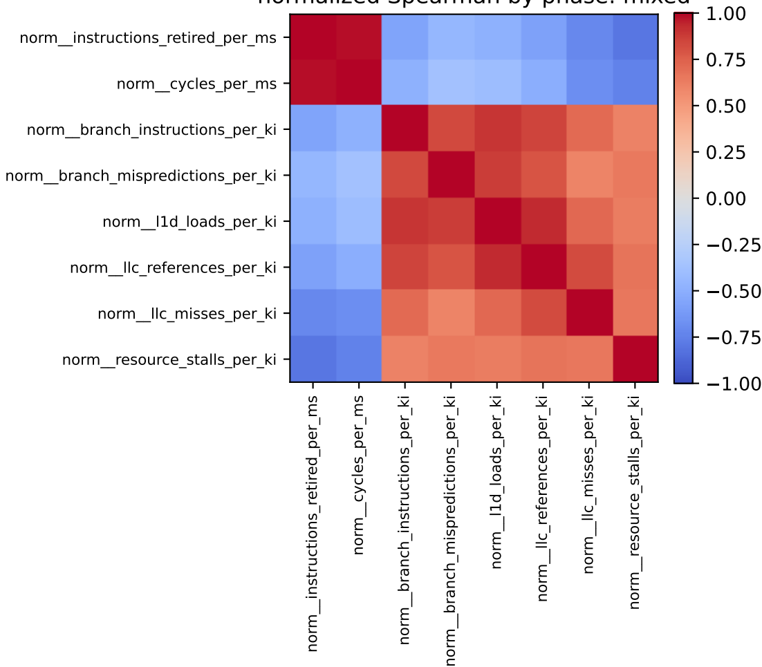
normalized Spearman by phase: mixed
