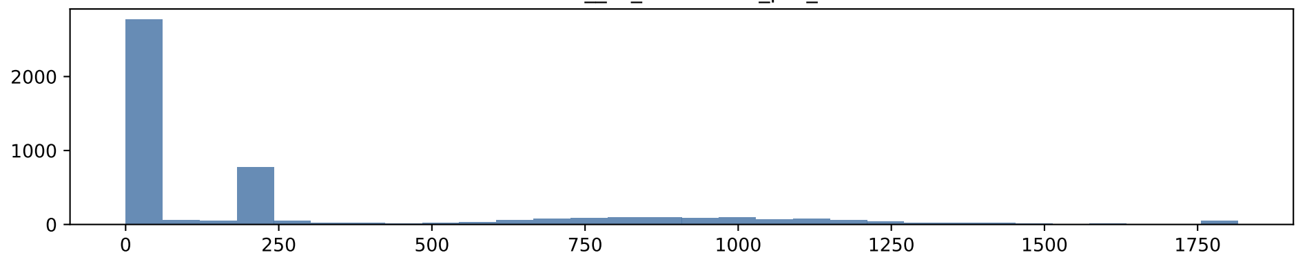
norm_llc_references_per_ki
