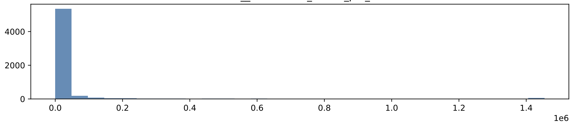
norm_cycles_per_ms
