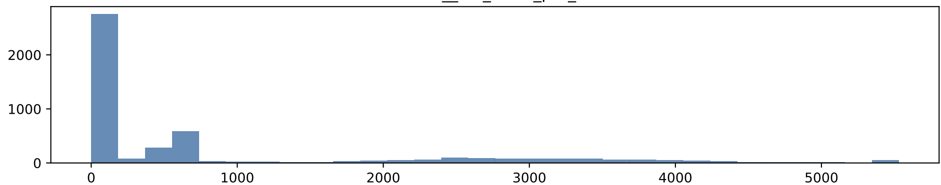
norm_l1d_loads_per_ki
