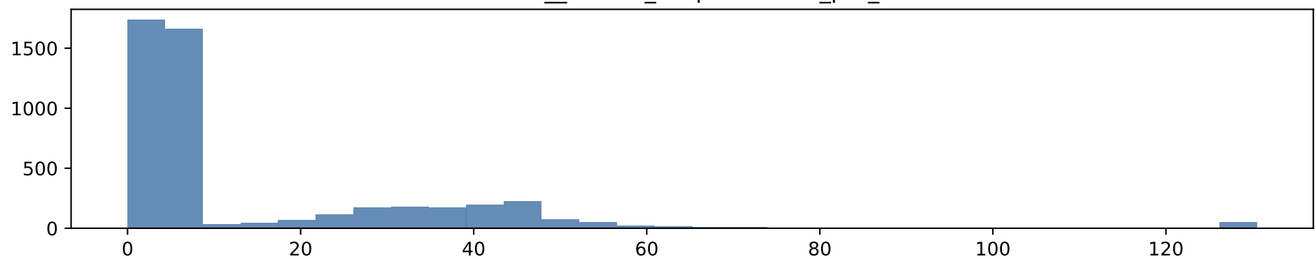
norm_branch_mispredictions_per_ki
