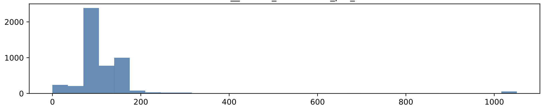
norm_branch_instructions_per_ki
