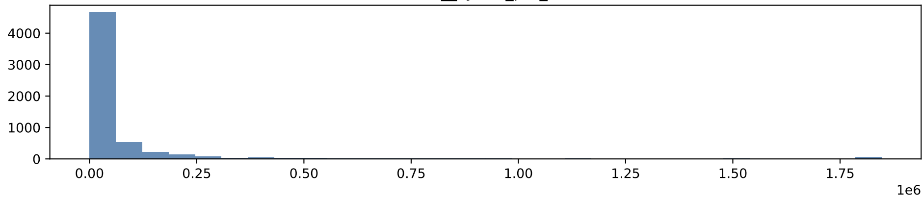
norm_branch_instructions_per_ki
