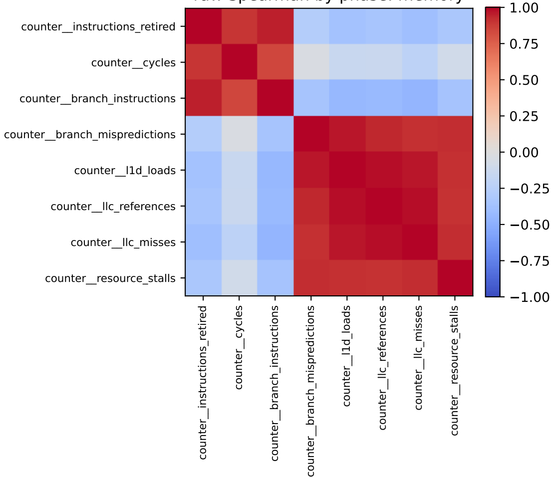
raw Spearman by phase: memory
