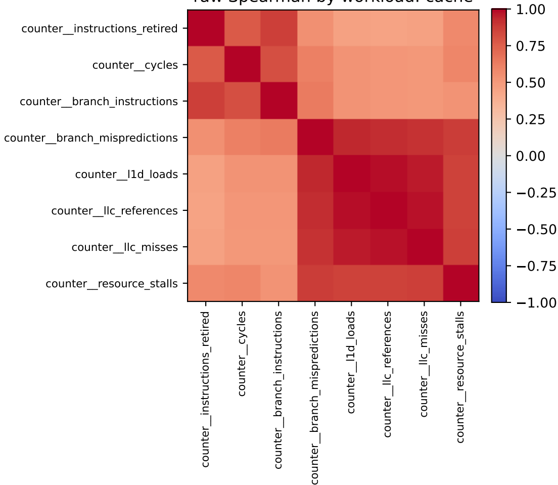
raw Spearman by workload: cache
