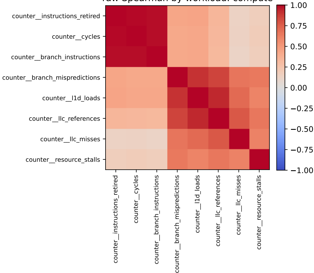
raw Spearman by workload: compute
