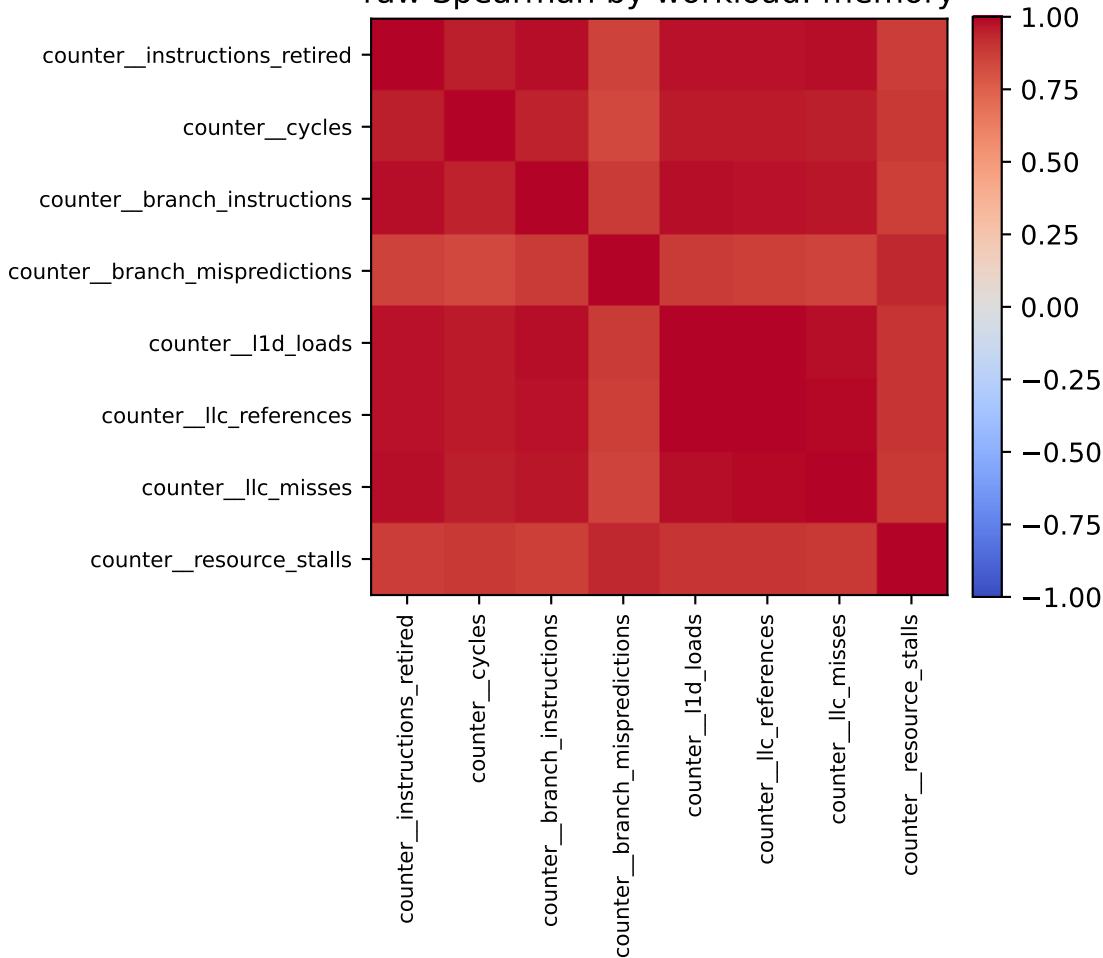
raw Spearman by workload: memory
