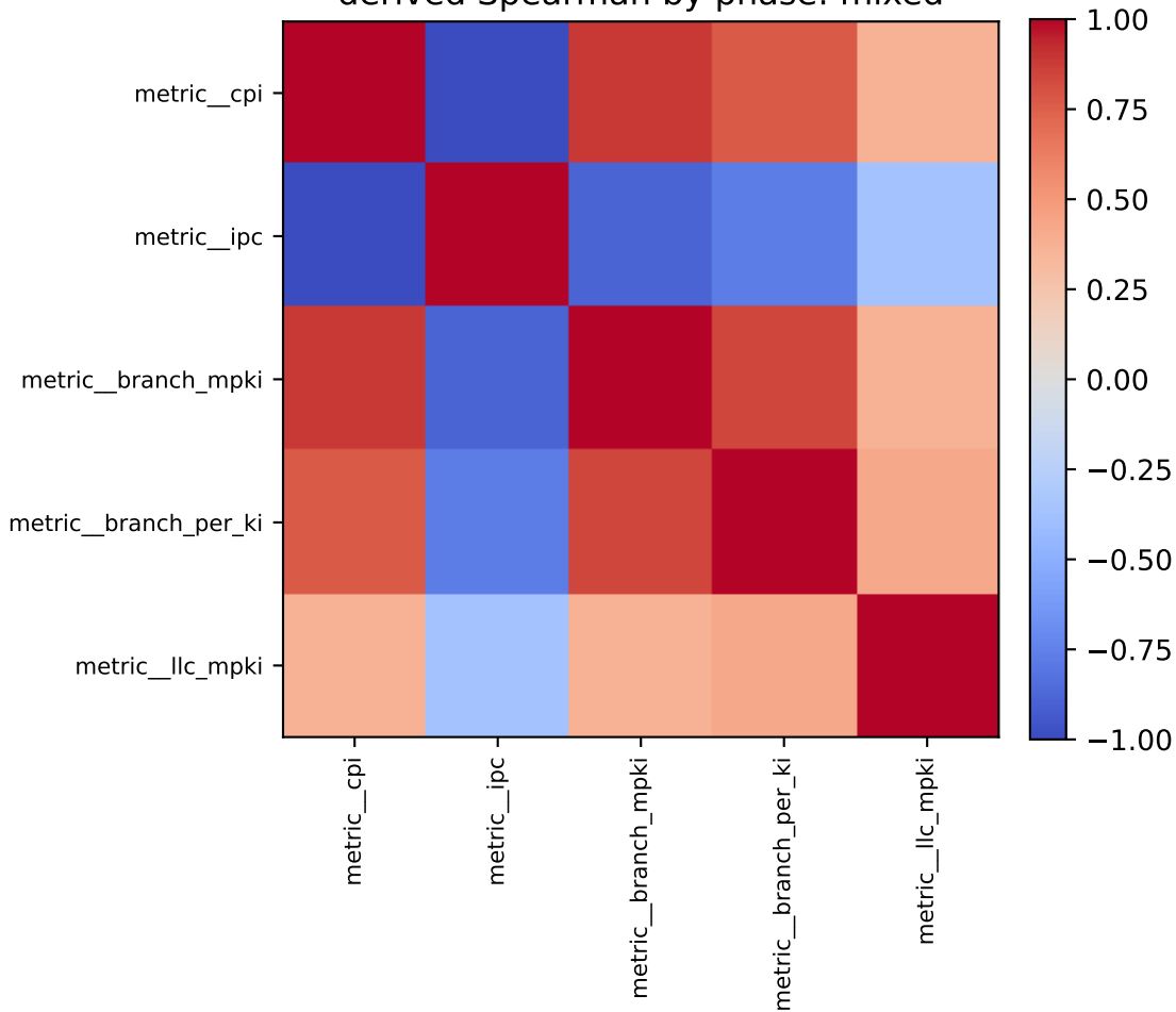
derived Spearman by phase: mixed
