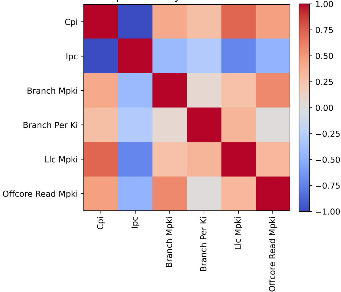
derived Spearman by workload: blackscholes
