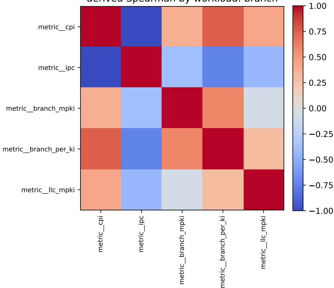
derived Spearman by workload: branch
