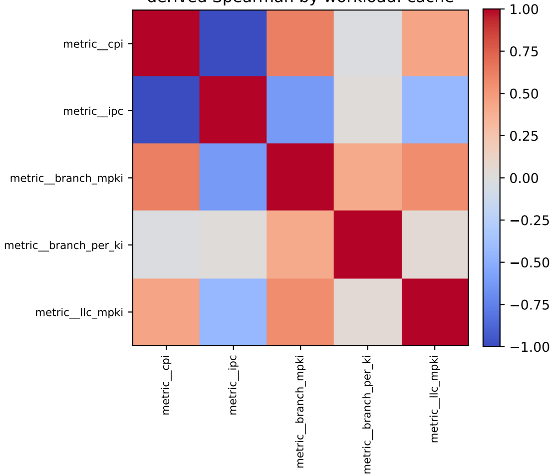
derived Spearman by workload: cache
