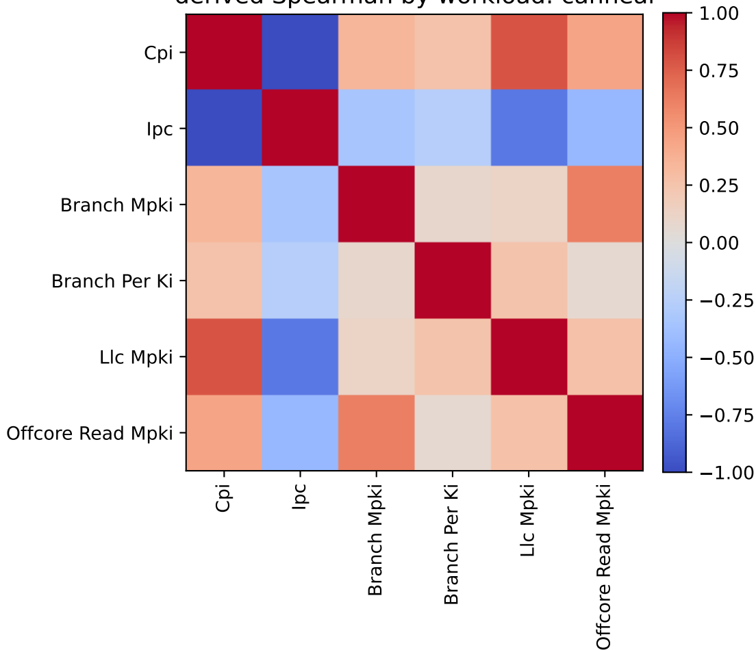
derived Spearman by workload: canneal
