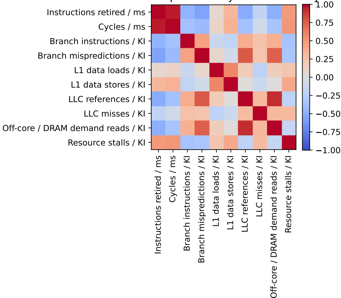
normalized Spearman by workload: bodytrack
