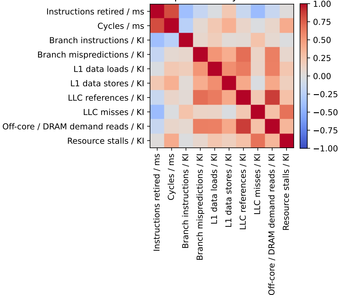
normalized Spearman by workload: canneal
