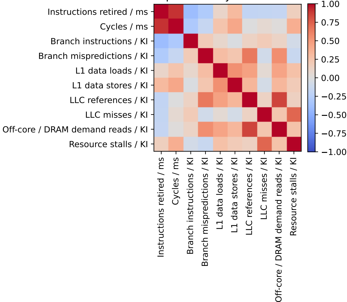
normalized Spearman by workload: fluidanimate
