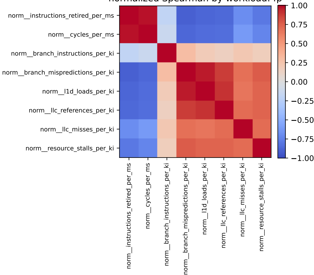
normalized Spearman by workload: fp
