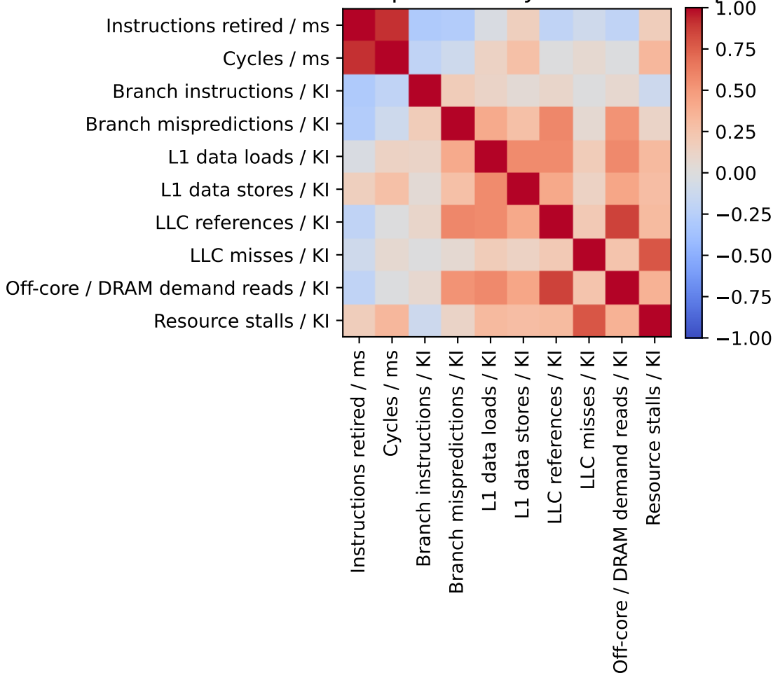
normalized Spearman by workload: freqmine
