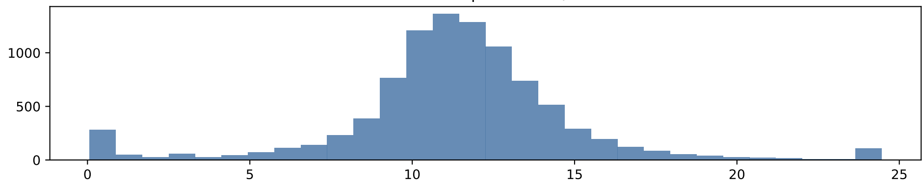
Branch mispredictions / KI
