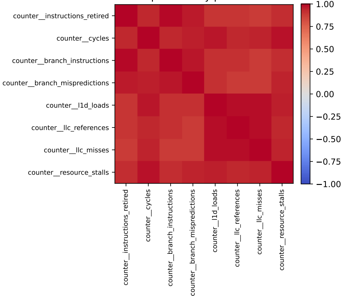
raw Spearman by phase: branch
