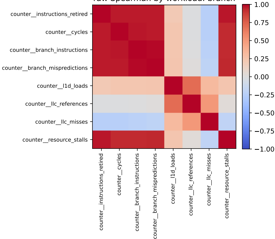
raw Spearman by workload: branch
