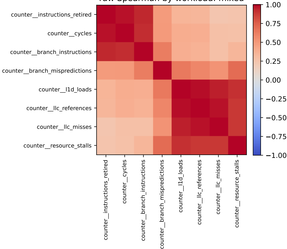
raw Spearman by workload: mixed
