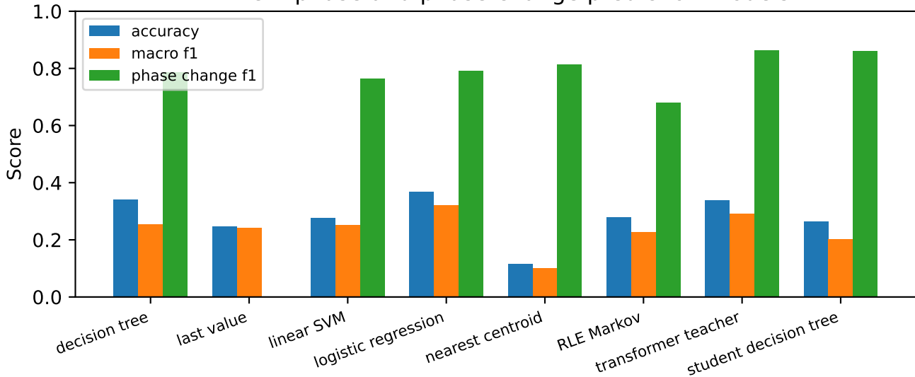
All next-phase and phase-change prediction models
